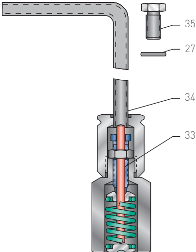
THREADED CAP AND GAG
